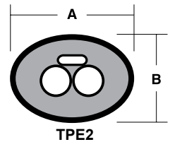
TPE2 - TWO 1/2" (12mm) PROCESS LINES WITH LOW TEMPERATURE TRACER
